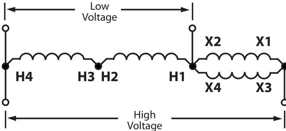
FIGURE 3 - Buck Boost Wiring Diagram
